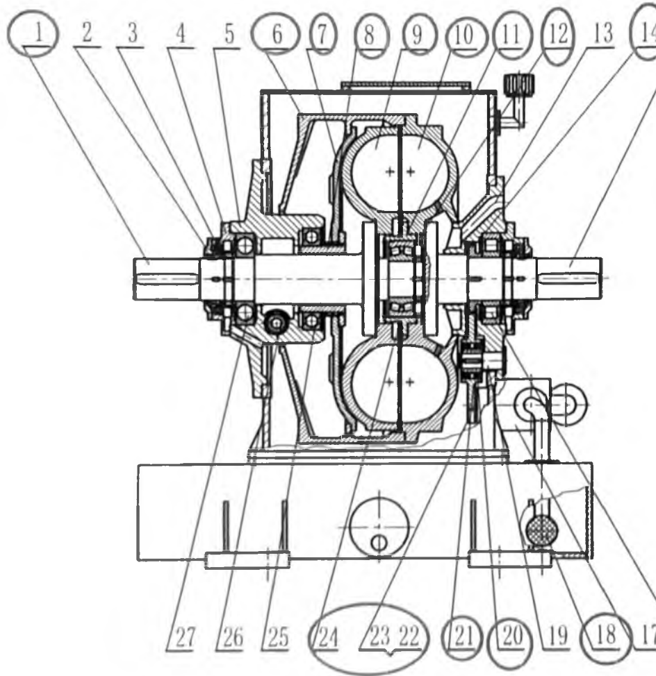
Fig. 5 YOTC \frac{1150}{1250} B Structure Drawing (NB5-C250F)
